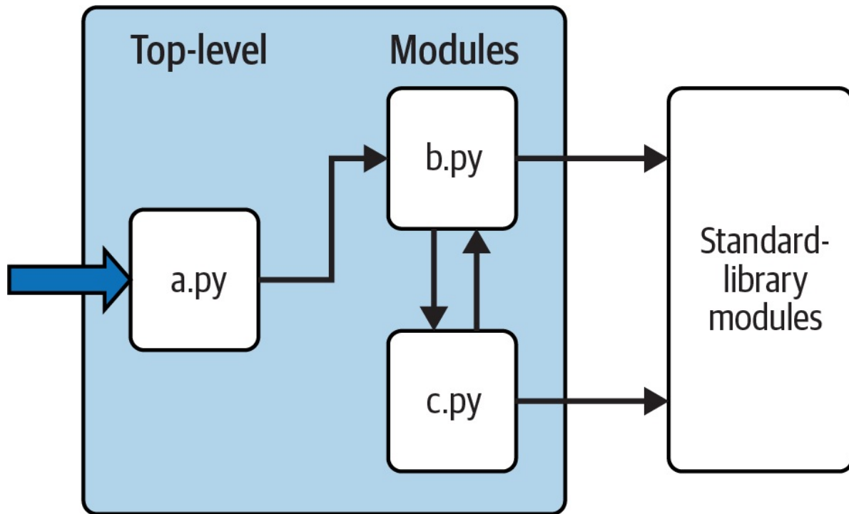
Figure 22-1. Program architecture in Python
