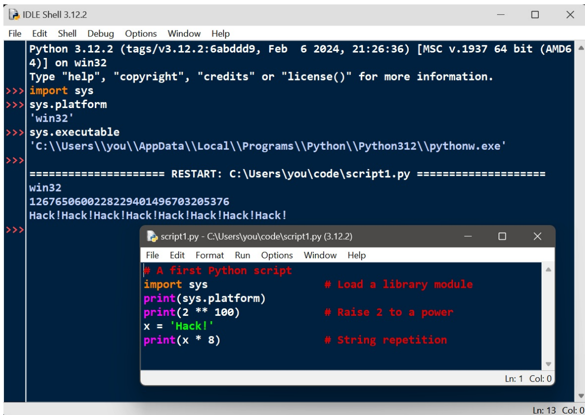
Figure 3-1. IDLE with its dark theme on Windows
