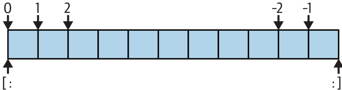
Figure 7-1. Indexes and slices: positives start from the left (0) and negatives from the right (-1)
